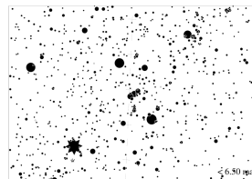
○Magnitude 6 Karte
