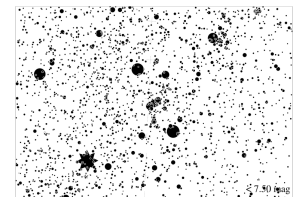
○Magnitude 7 Karte
