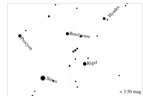
○Magnitude 3 Karte
