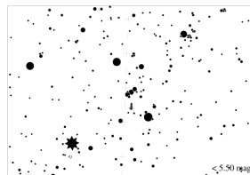
○Magnitude 5 Karte
