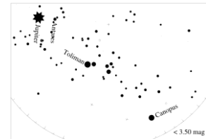
3 Magnitude 3 Chart
